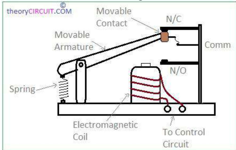
Figure 2.4: Relay Diagram
