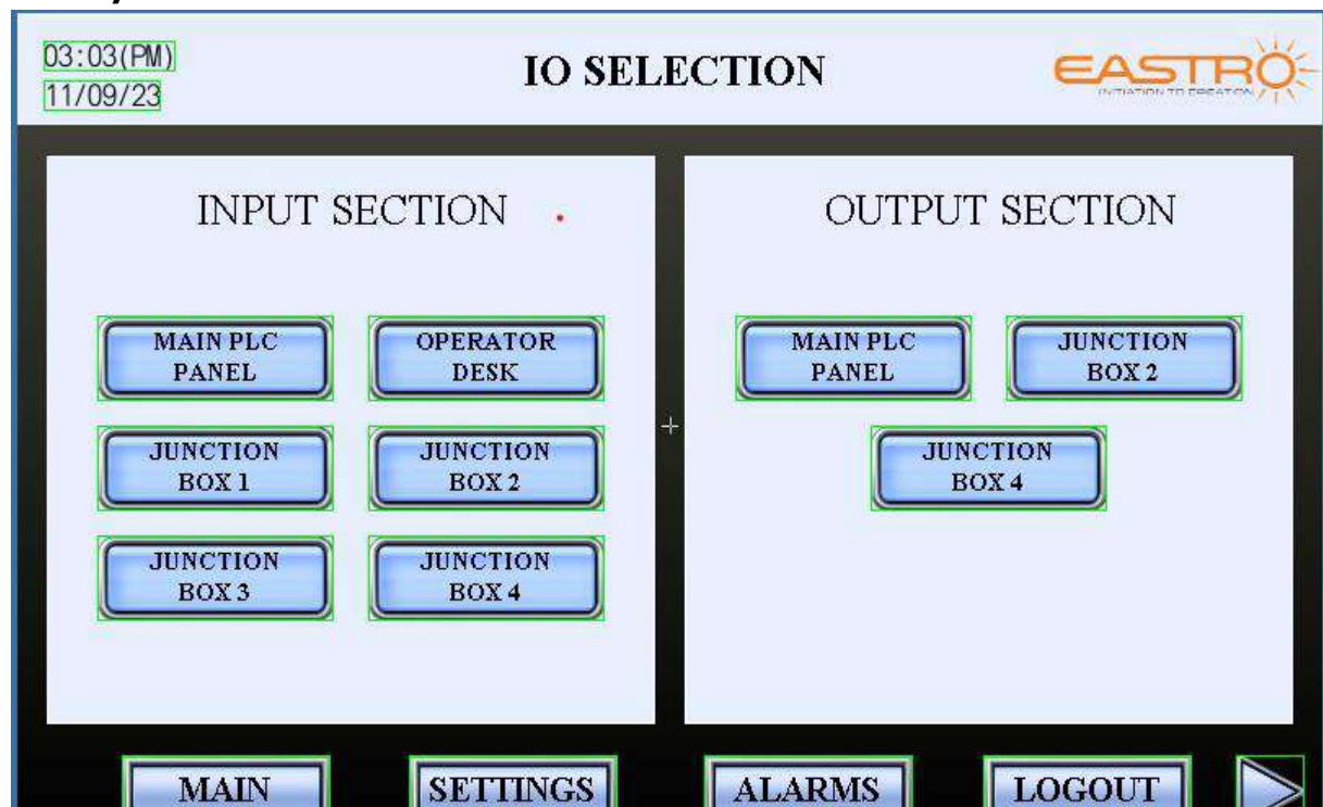
Fig 2.5. HMI screen-2
