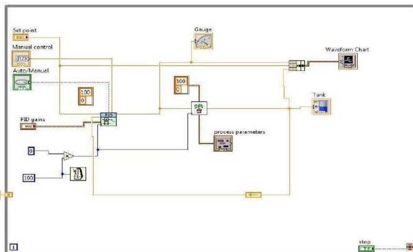
Figure 3.2.2. Block diagram liquid level control
